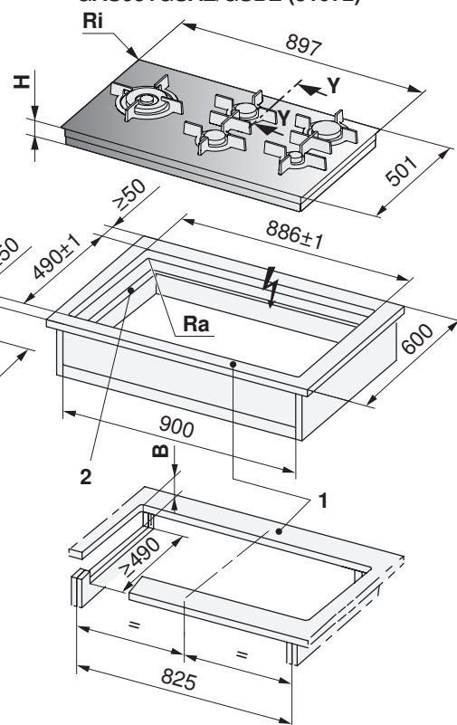
GAS951GSAZ/GSBZ (31072)
